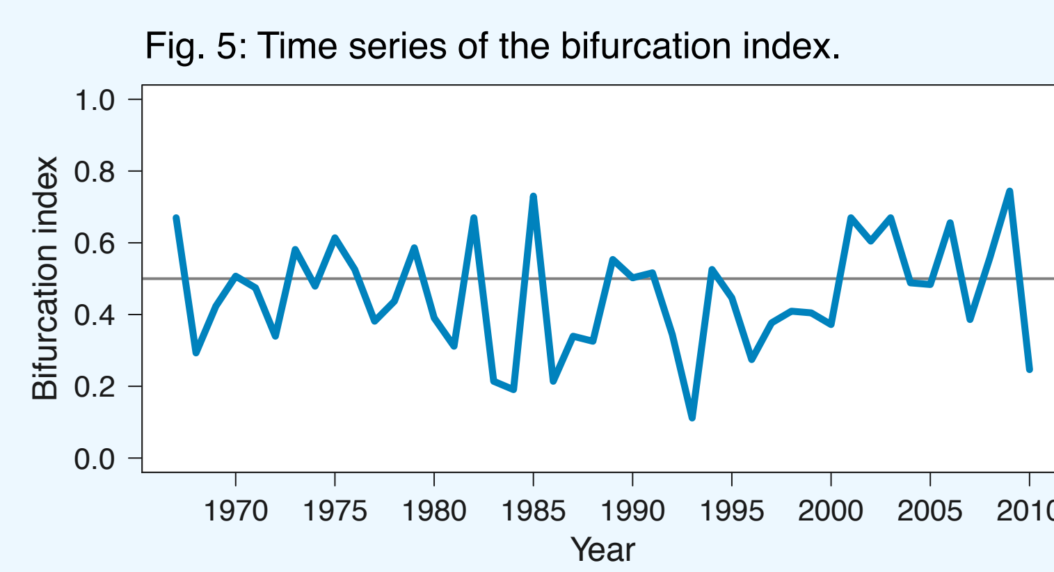
Fig. 5: Time series of the bifurcation index.
