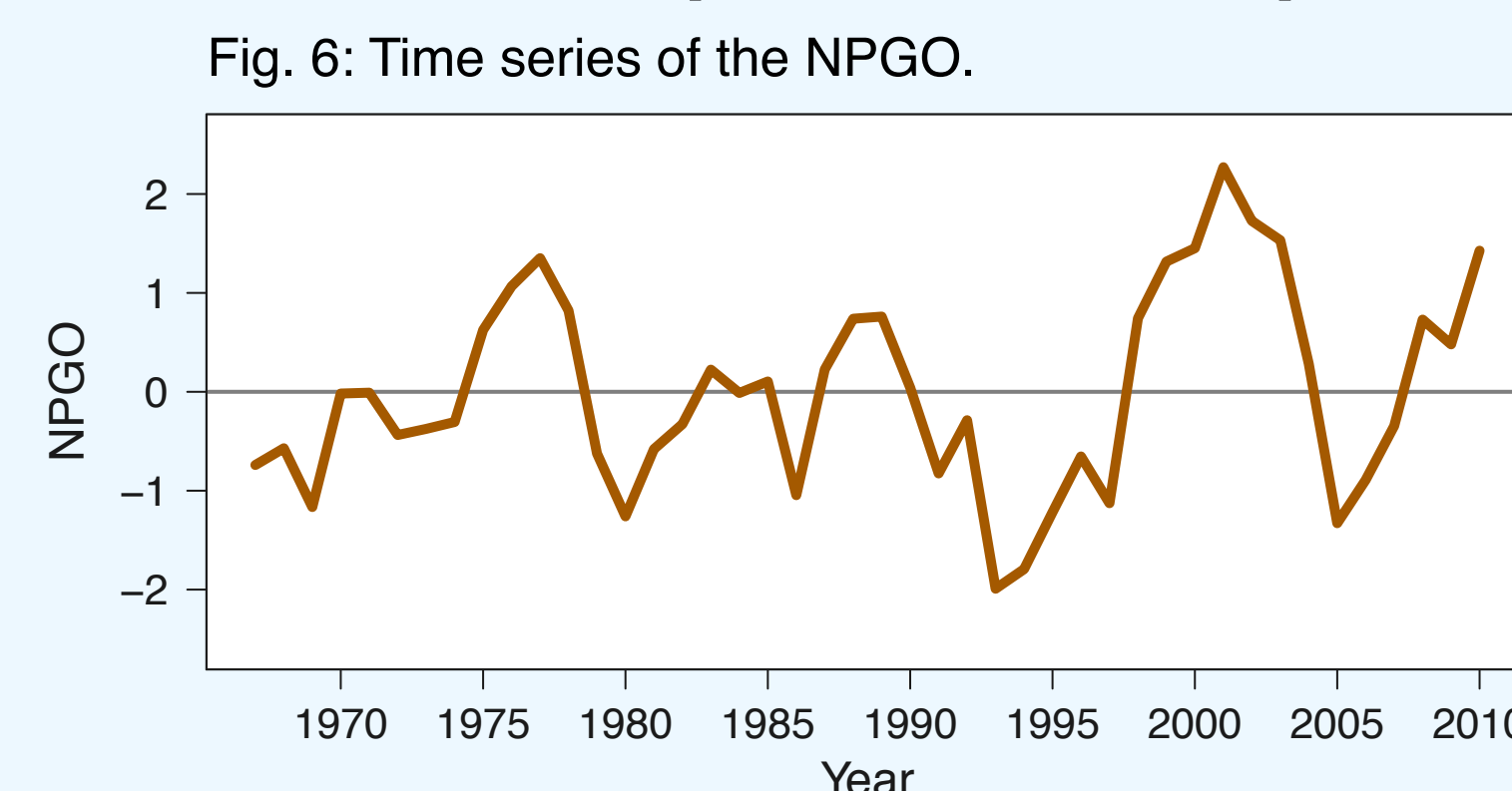
Fig. 6: Time series of the NPGO.
